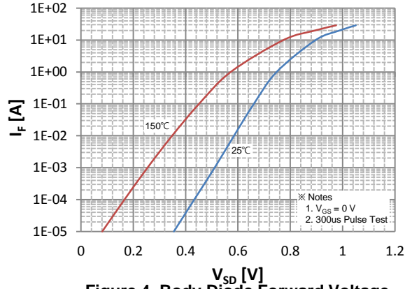
V SD [V] Figure 4. Body Diode Forward Voltage Variation with Source Current and Temperature
