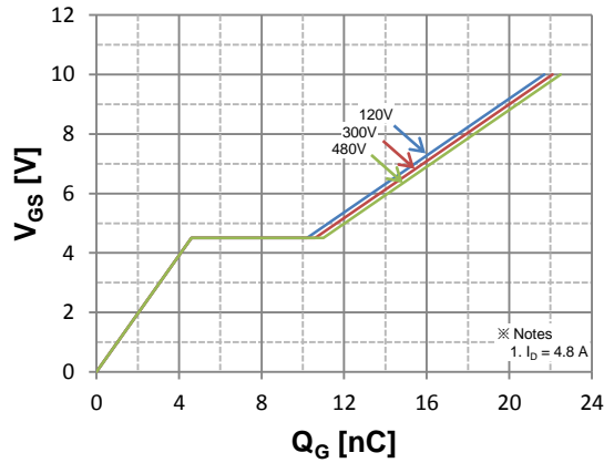
Q G [nC] Figure 6. Gate Charge Characteristics
