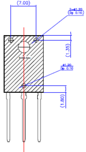
BTM VIEW
